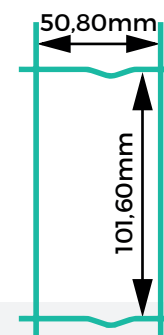
POTEAU T
